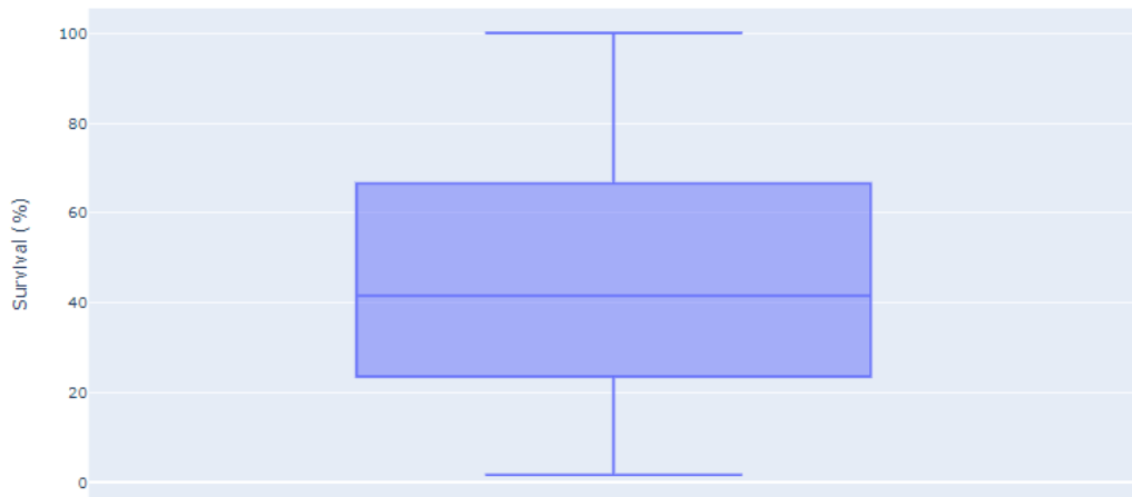
Figure 4.59: outlier box plot.
