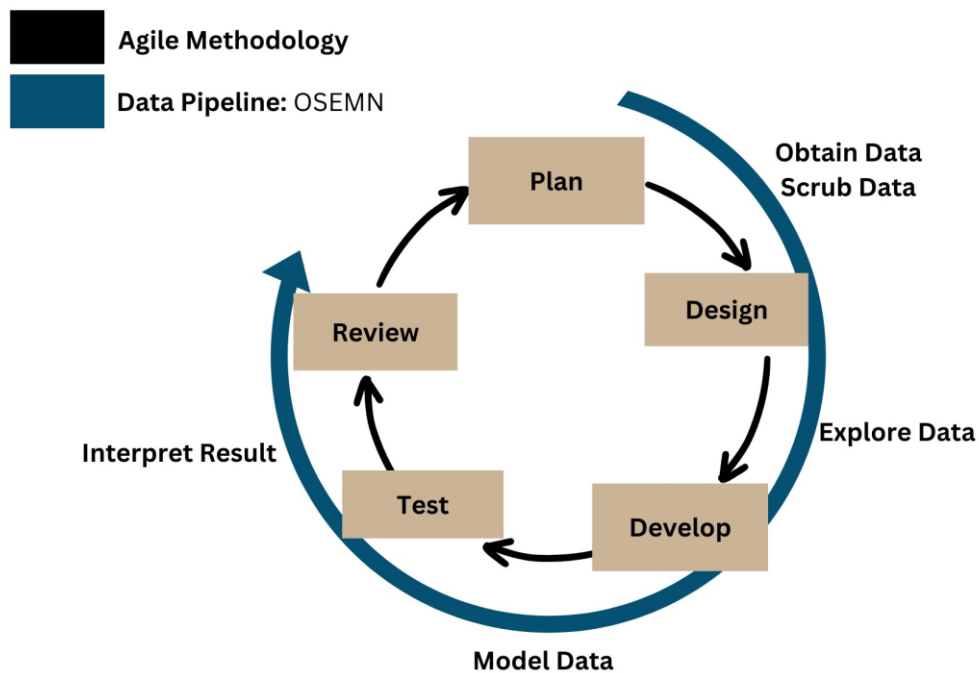
Figure 3.1 Methodology in CANCERVIVE
